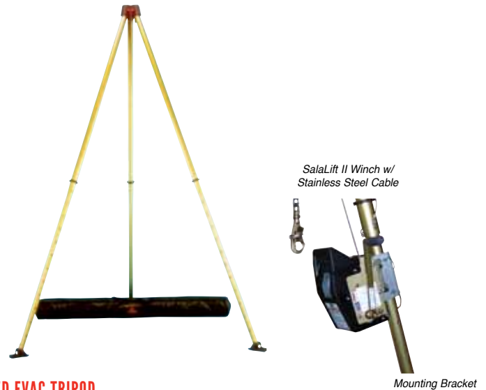
Mounting Bracket
