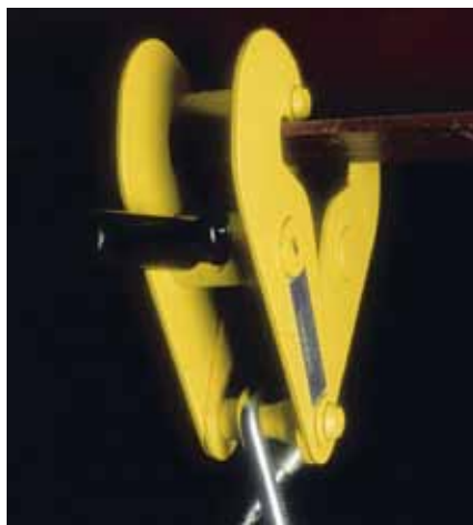
Actuated Girder Grip ready for insertion
