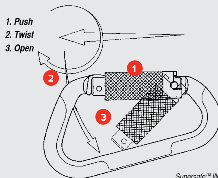
Supersafe™ Illustration
