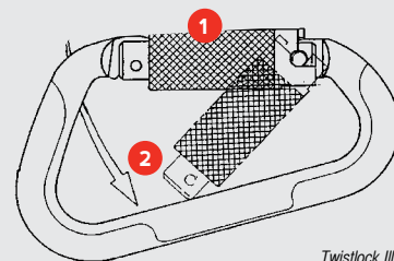
Twistlock Illustration
