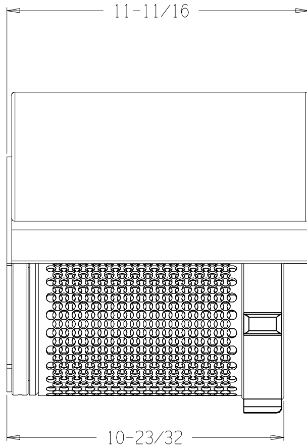
SIDE VIEW
